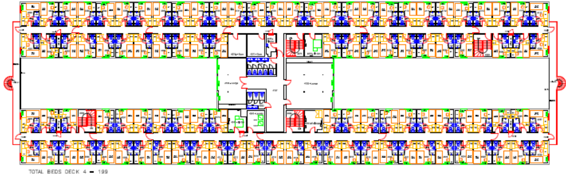
PLAN VIEW ON DECK 4 SCALE 1:150
